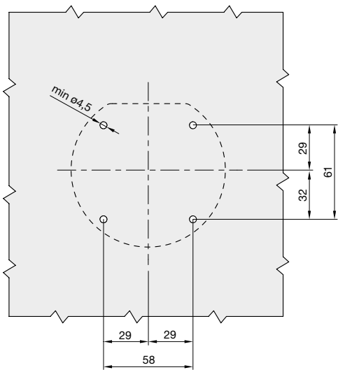
Drilling template for front fixing
