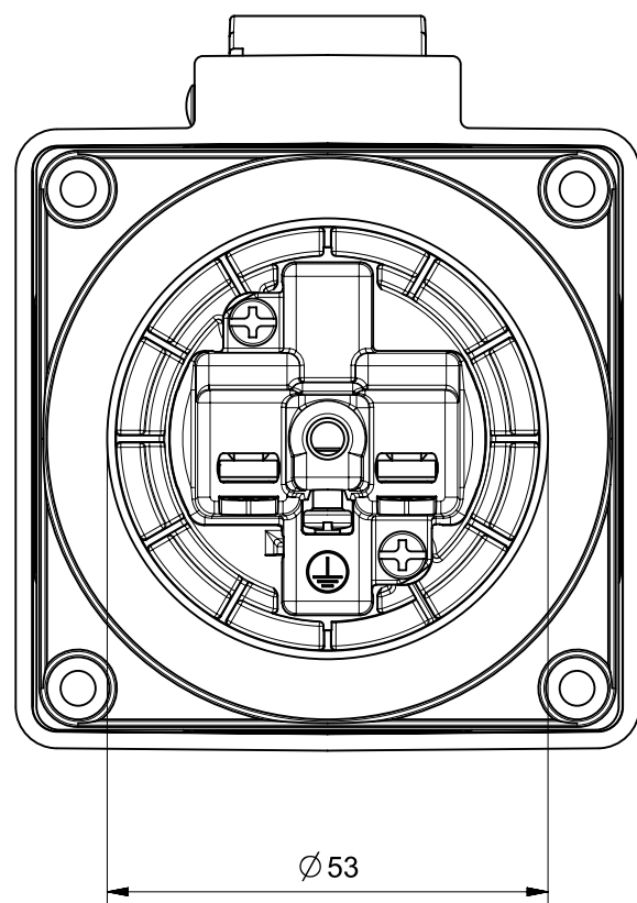
DIAMETRO FORATURA PANNELLO PANEL DRILLING HOLE
