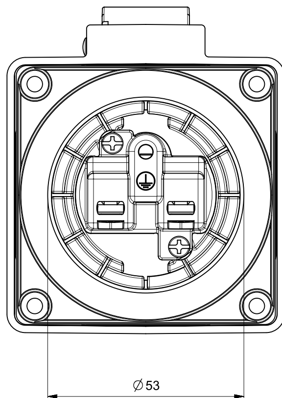
DIAMETRO FORATURA PANNELLO PANEL DRILLING HOLE
